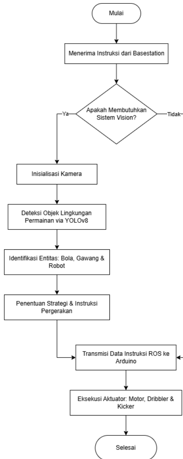
Gambar 2.3 Flowchart Kerja Robot KRSBI Beroda
