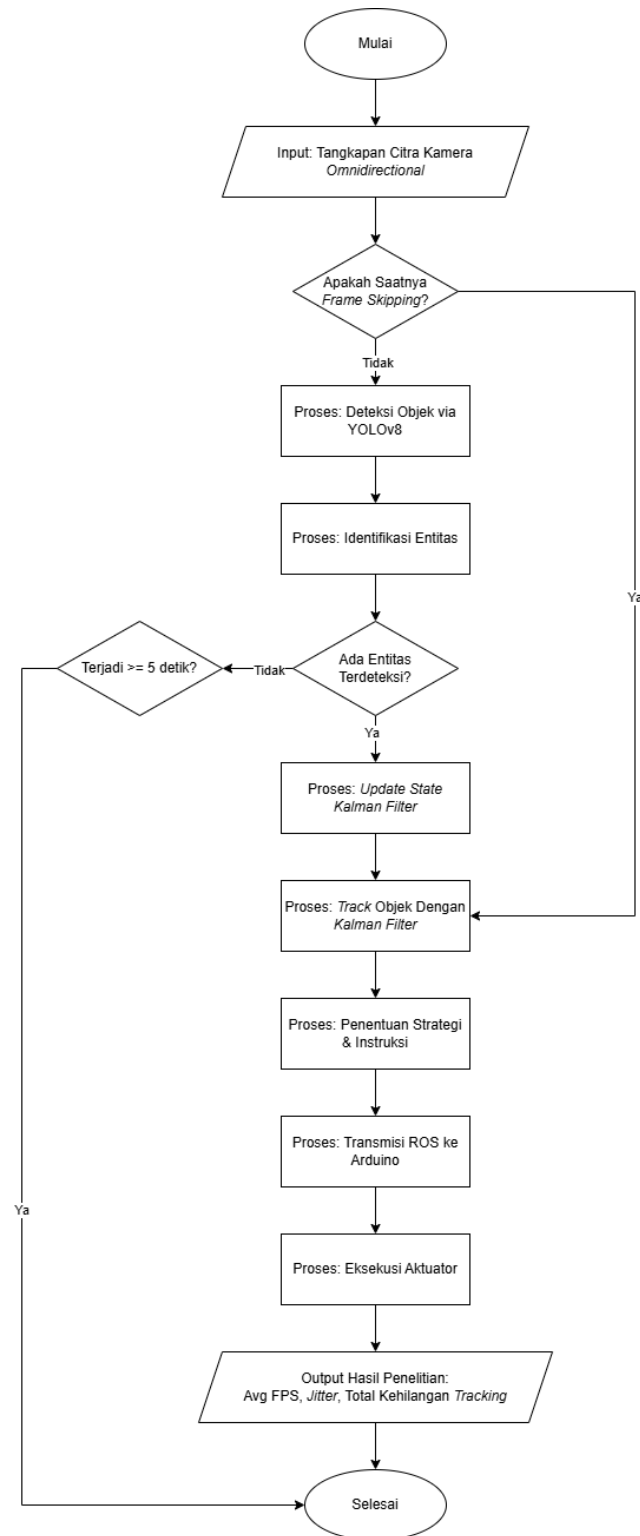
Gambar 3.4 Flowchart Kerja Sistem Optimized
